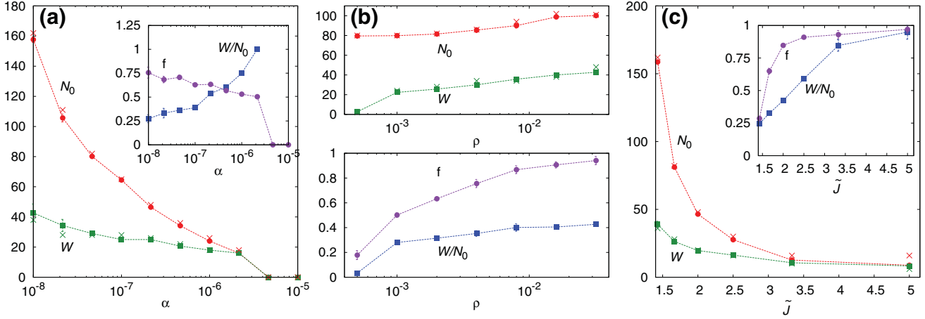
FIG. 3. (Color online) (a) Dependence of the steady-state most-likely cluster size N_0 (red circles) and the full width at half maximum W (green squares) of the cluster-size distribution vs the proteolytic rate \alpha . Crosses ( \times ) indicate corresponding values derived from fluxes near N_0 via Eq. (2). The inset shows the relative width W/N_0 (blue squares) and the fraction of G proteins in large domains (purple circles) vs \alpha . Error bars indicate statistical errors, which are often smaller than point sizes. Other parameters are \tilde{J} = 1.67 and \rho = 2 \times 10^{-3} . (b) The top figure shows size N_0 (red circles) and width W (green squares) vs average membrane density \rho \equiv N_g/L^2 . The bottom figure shows the dependence of relative width W/N_0 (blue squares) and the cluster fraction f (purple circles). Other parameters: \tilde{J} = 1.67 and \alpha = 5 \times 10^{-8} . (c) Size N_0 (red circles) and width W (green squares) vs the clustering interaction \tilde{J} \equiv J/(k_B T) . The inset shows the relative width W/N_0 (blue squares) and the fraction of G proteins in large domains f (purple circles) vs \tilde{J} . Other parameters: \rho = 2 \times 10^{-3} and \alpha = 5 \times 10^{-8} .
