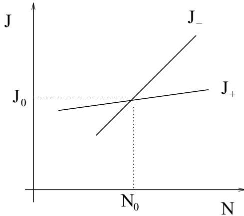
FIG. 5. Mean-field fixed-point cluster size N_0 that occurs where the evaporative and condensative fluxes are equal ( J_- = J_+ = J_0 ). The fixed point is stable when evaporation is stronger than condensation ( J_- > J_+ ) for N > N_0 , as illustrated. The demonstration of monotonicities in Appendix B are for N \approx N_0 , where a linear approximation for J_{\pm} holds.
