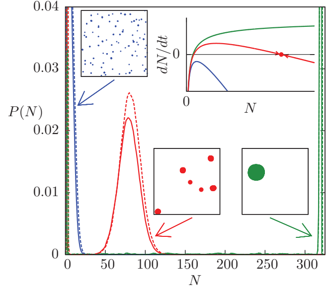
FIG. 2. (Color online) Cluster-size probability distribution, P(N) , vs number of monomers in a cluster, N , for low ( \alpha = 10^{-9} , green, right), medium ( \alpha = 5 \times 10^{-8} , red, center), and high ( \alpha = 10^{-5} , blue, left) proteolytic rates (per protein per time step, where \Delta t \approx 10^{-4} s). Other parameters are \tilde{J} = 1.67 and \rho = 2 \times 10^{-3} . The dotted lines represent the reconstruction of the probability distribution via Eq. (2). Intermediate proteolytic rates stabilize a peaked steady-state cluster-size distribution with multiple large clusters, as illustrated by the corresponding snapshot of the system. The inset is a stability diagram from Eq. (1), illustrating the effects of low (green, top curve, with only an unstable fixed point), medium (red, center curve, with an additional stable fixed point as indicated), and high (blue, bottom curve, with no fixed points) proteolytic rates on the domain size dynamics dN/dt vs domain size N .
