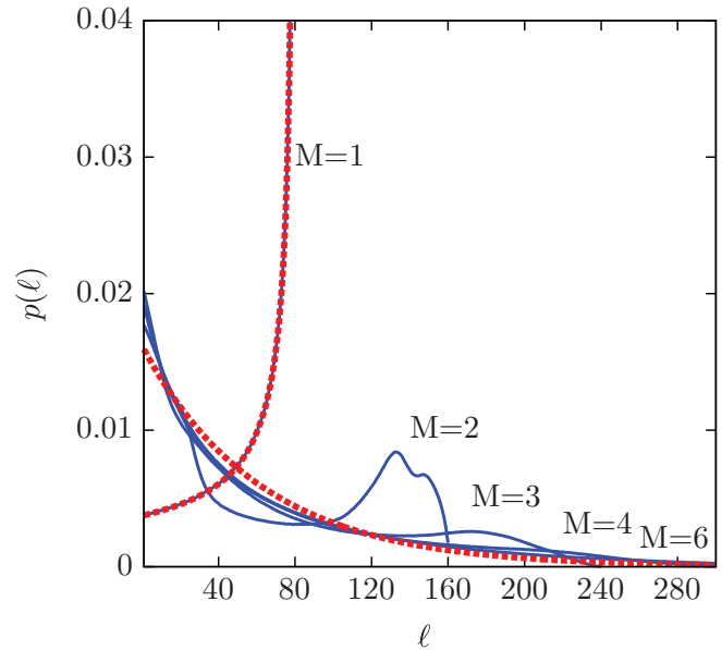
FIG. 4. (Color online) Probability distribution p_M(l) of the maximum length for various number of pili ( M = 1, 2, 3, 4, 6 ) sharing the same common pool of monomers. We use t = 0.3 and N_p = 40 , though qualitatively similar results are seen with other parameters. The continuous lines are the result of the stochastic simulation. The red dashed lines represent the two exact limiting distributions p_1 and p_\infty , overlaying the M = 1 data and close to the M = 6 data, respectively.
